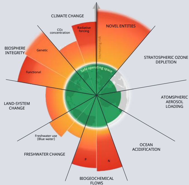
The 2023 update to the Planetary boundaries より一部抜粋
